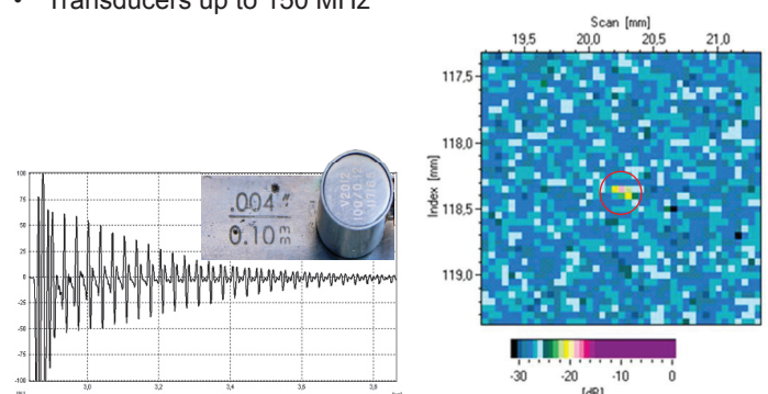
A-scan of a 0.1 mm thick feeler gauge
