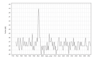
Echo dynamic curve of a 50 \mu\text{m} flat bottom hole (C-Scan is shown below)
