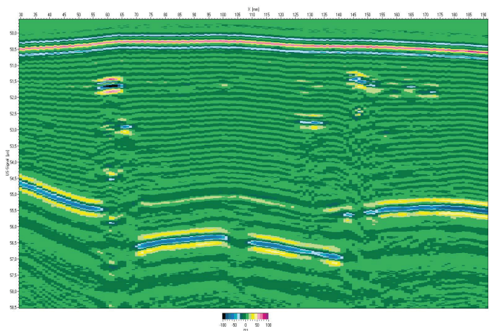
B-scan of a CFRP component with different thicknesses, indications of layers and delaminations
