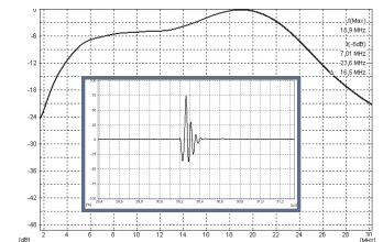
A 15 MHz probe delivers a -6 dB spectrum from 7.01 to 23.6 MHz
